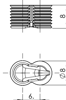
Fixi housing:
